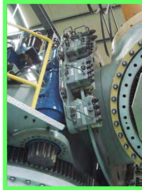
Brakes on low speed shaft
